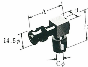
2図 BNC195-LP
